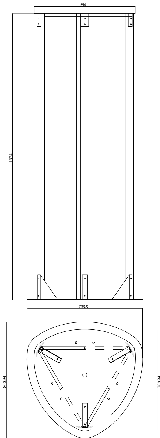
three-sided totem display frame h200x60
