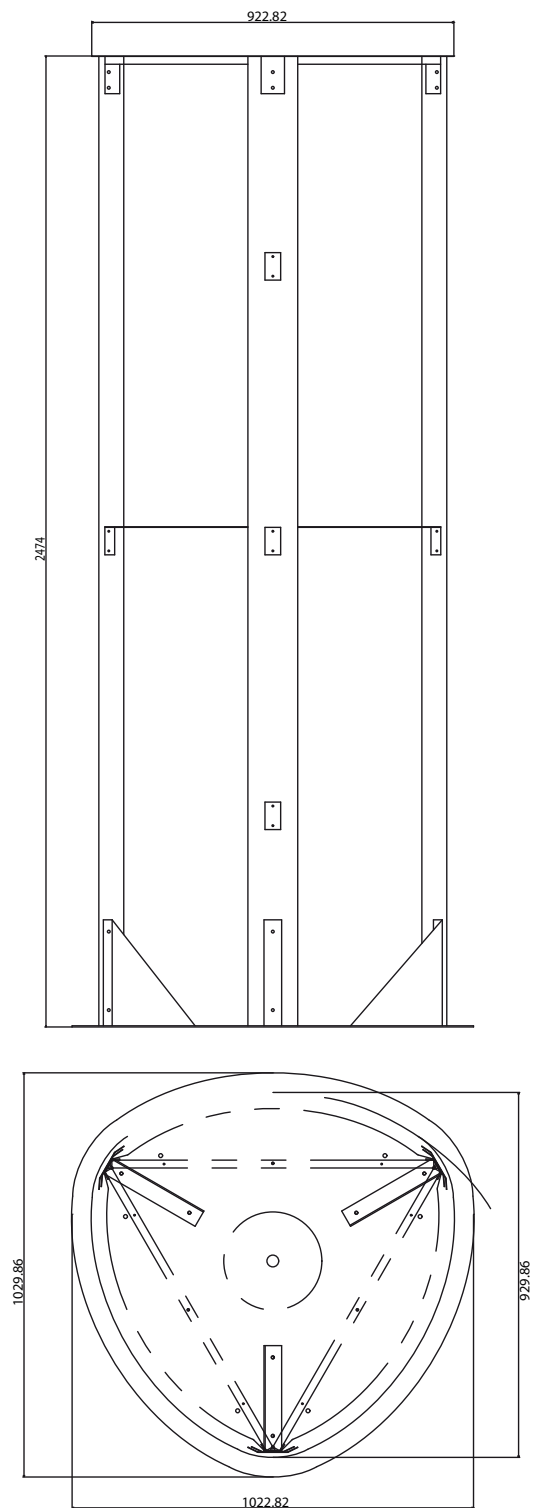
three-sided totem display frame H250x80
